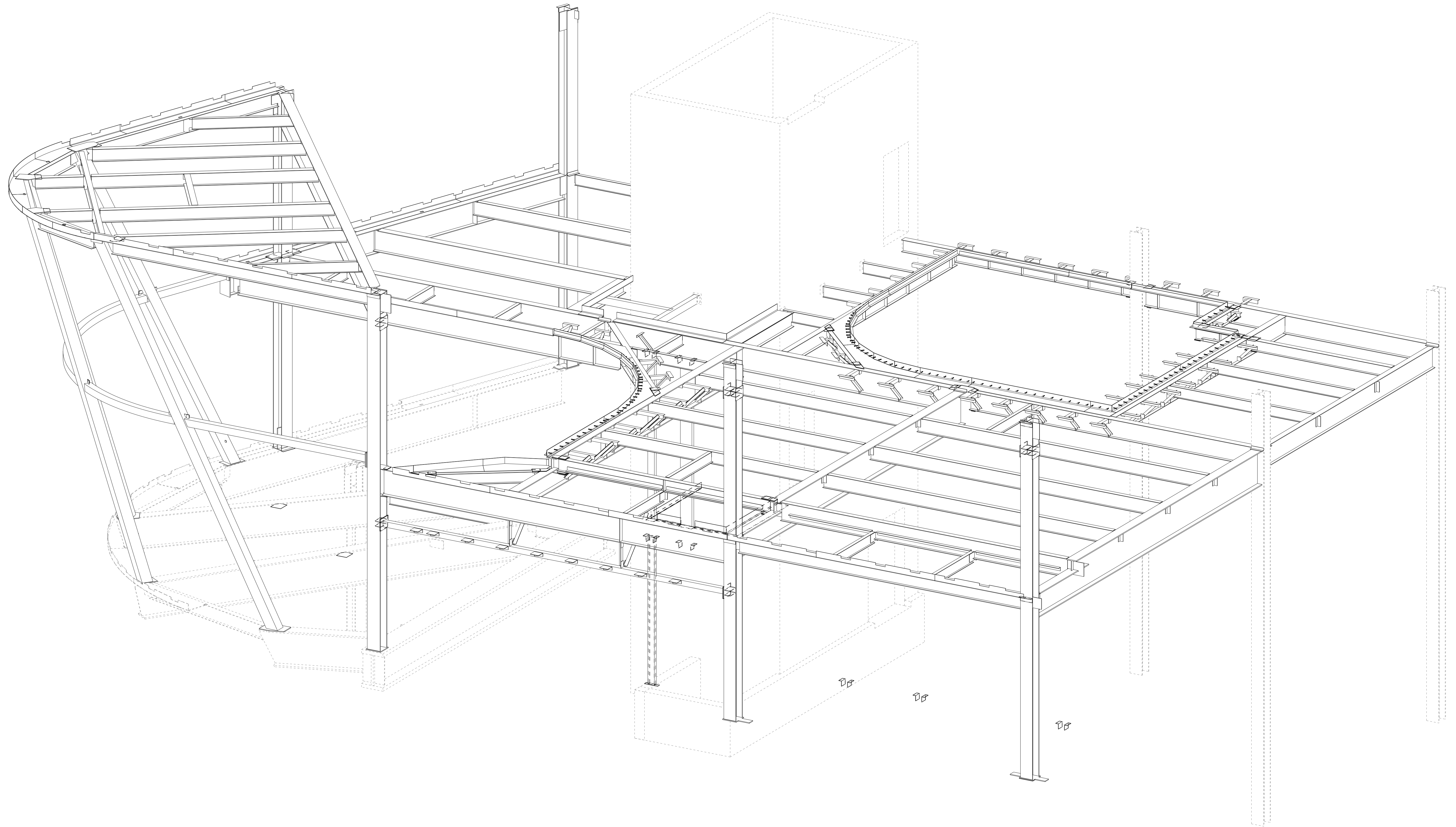
SEQ.#102 ISOMETRIC VIEW (REF.DWG.# S0-00)
